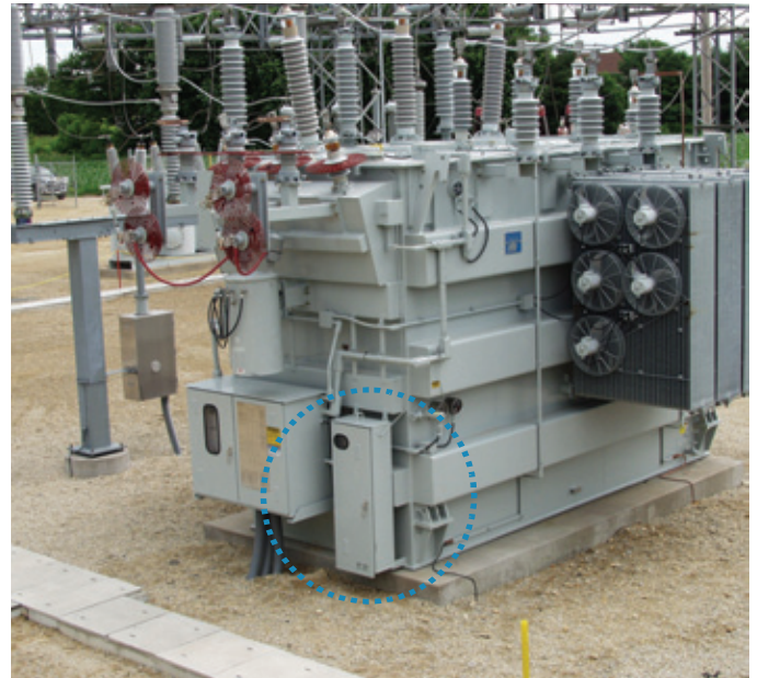
Supply and tank pressure gauges on the Inert Air System are easily viewed through a large viewing port on the cabinet door.
